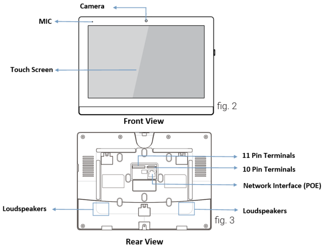
fig. 2: front view
